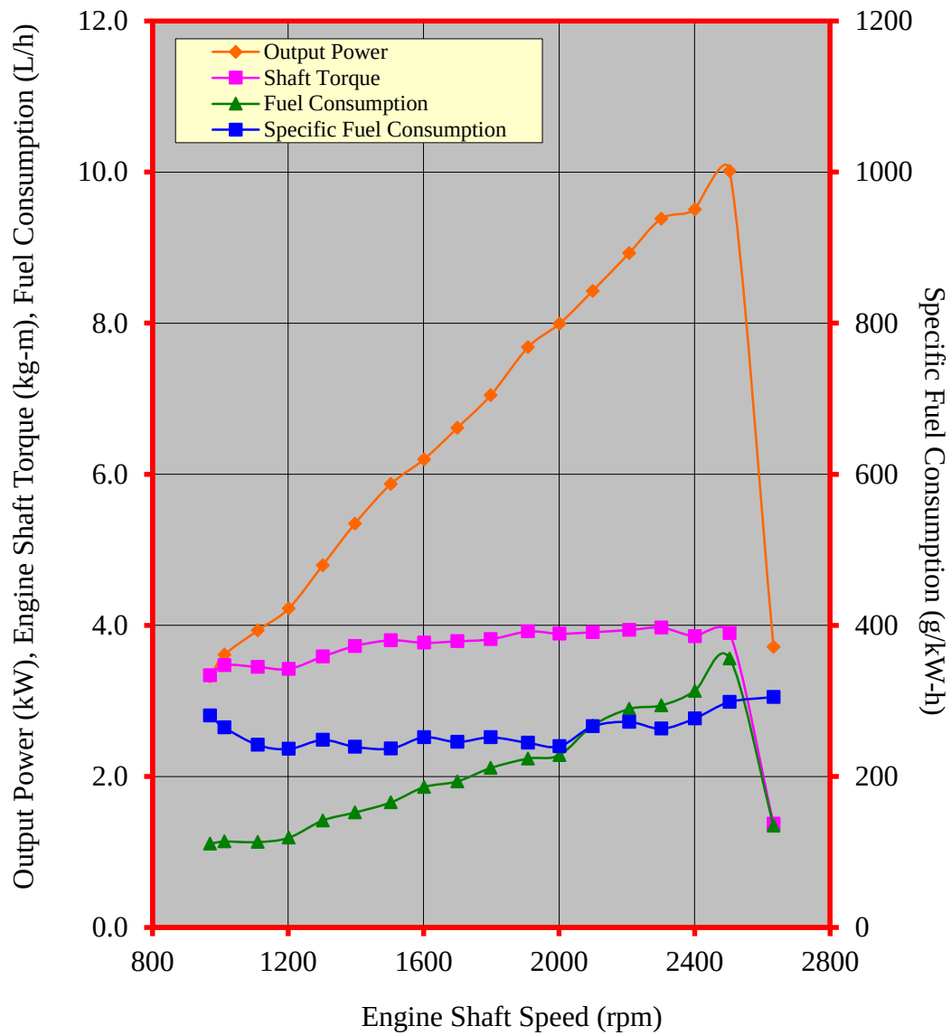
Figure 3. Performance characteristic curves of the PLATINUM PT140DI KNM140 diesel engine
