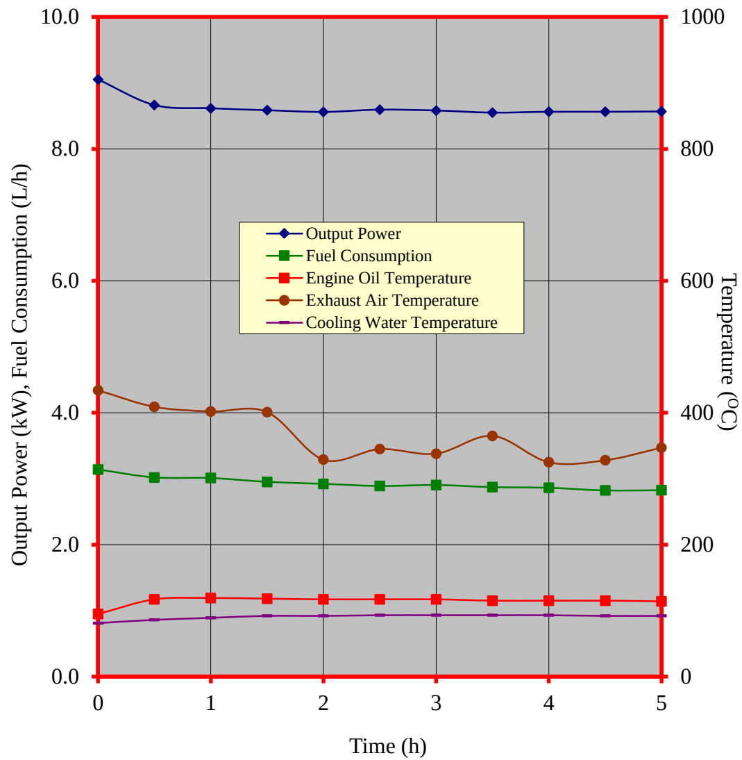
Figure 4. Performance characteristic curves during the continuous running test of the PLATINUM PT140DI KNM140 diesel engine
